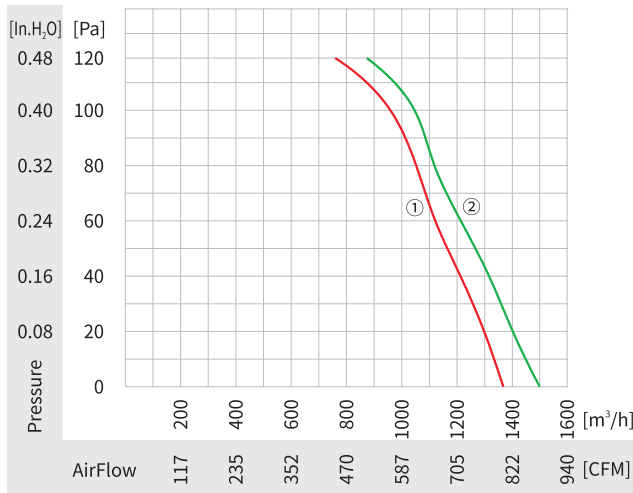
2-Pole
