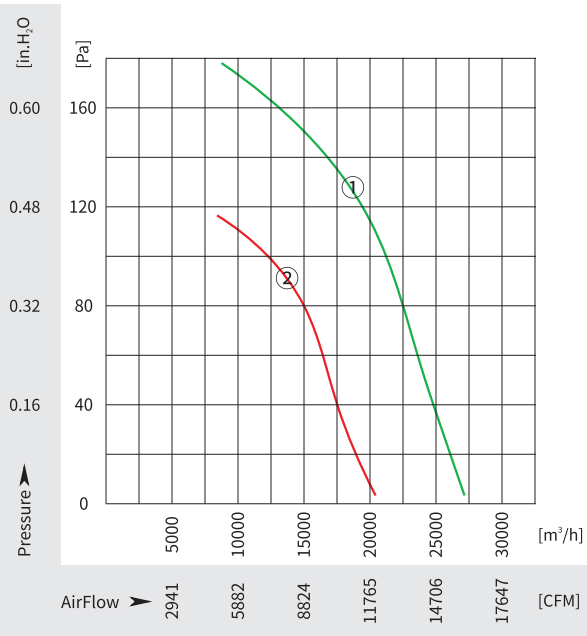
6-Pole
