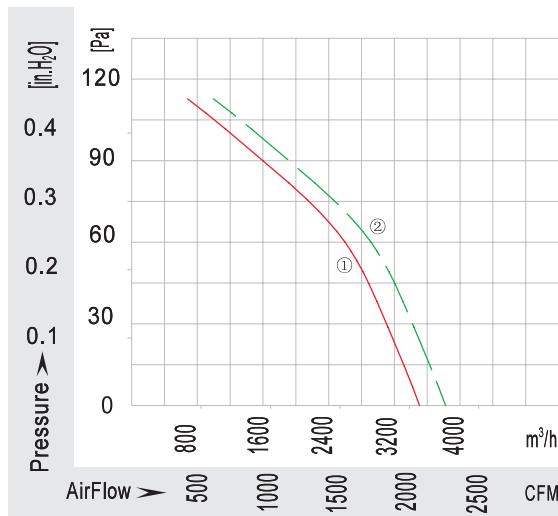
4-Pole
