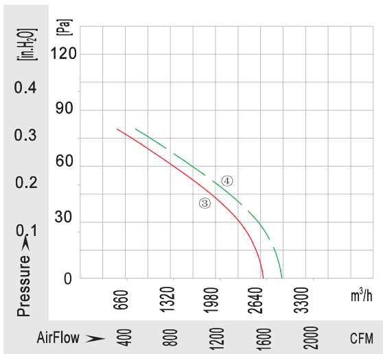
6-Pole
