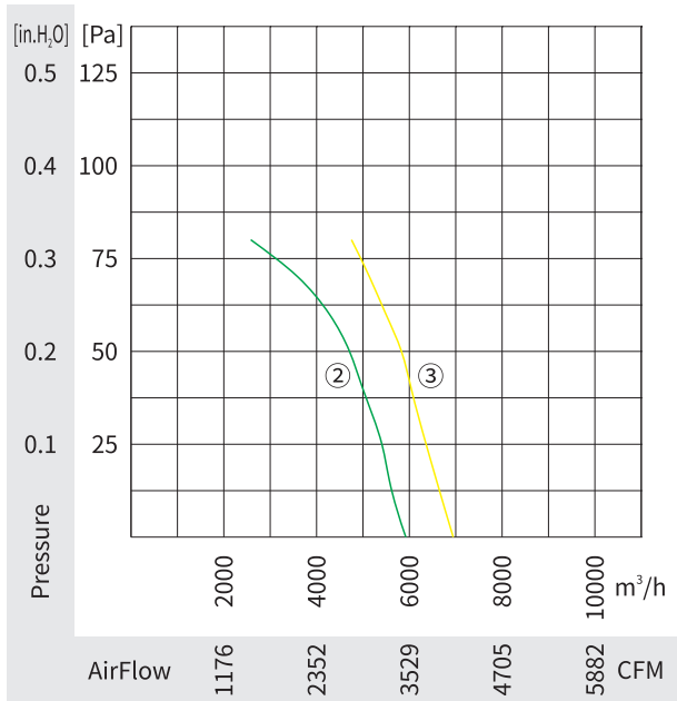
6-pole
